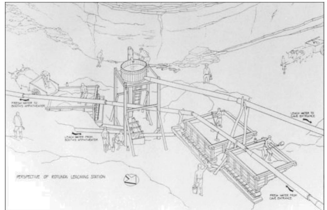
Diagram showing saltpeter mining operation in a cave. www.nashvillefossils.com
